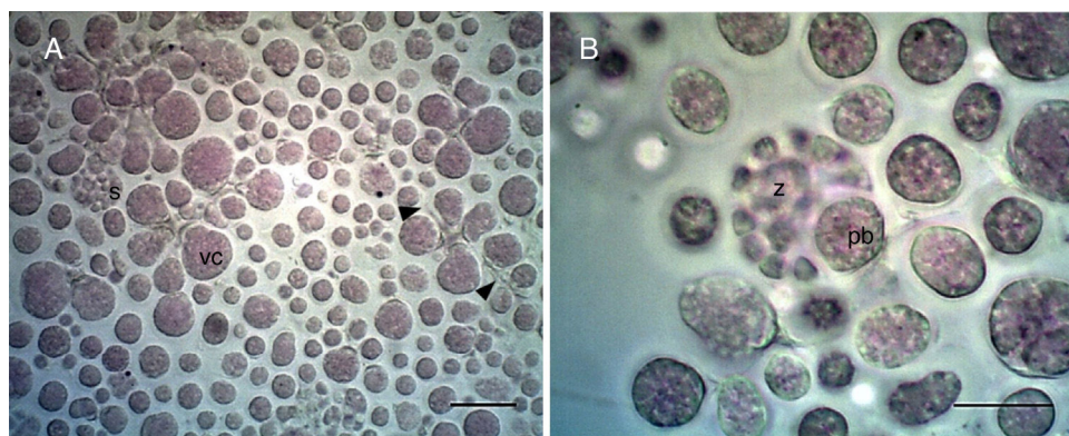
Fig. 1 – Light microscopy of cells in Antarctic strain 34-2 stained with methyl violet. A Vegetative cells (vc), sporangia (s) and ectoplasmic nets (arrows). Scale bar 100 \mu m. B Mature sporangium with zoospores (z) and proliferative body (pb). Scale bar 50 \mu m.
