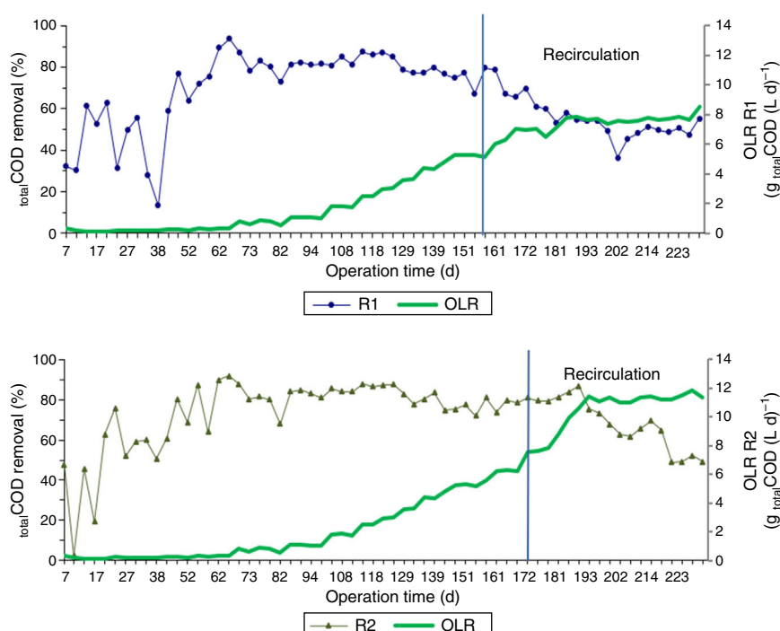
Figure 5 – Removal efficiency of the total chemical oxygen demand ( \text{totalCOD} ) as a function of the organic loading rate (OLR) applied in the UASB reactors (R1 and R2) for vinasse treatment.
