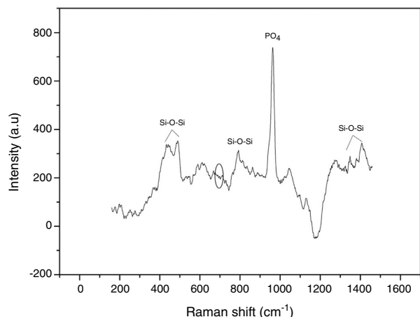
Figure 3 – Raman spectrum of synthesized VC after 600 °C heat treatment.
