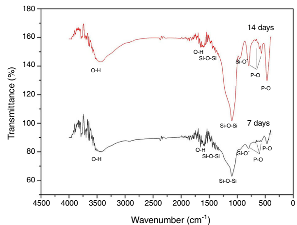
Figure 8 – FTIR analysis of formed layer on VC surface after 7 and 14 days in SBF.
