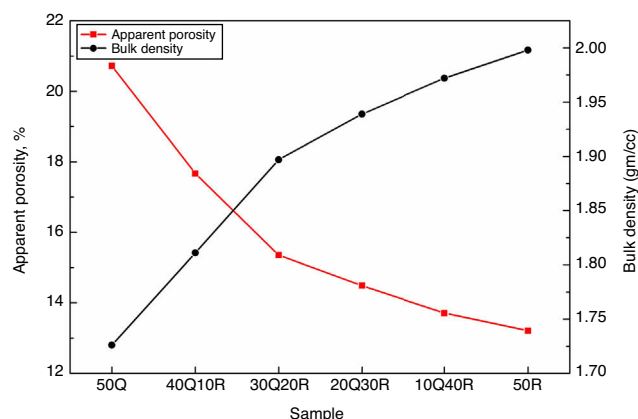
Fig. 3 – Apparent porosity and bulk density of samples sintered at 1200 °C.
