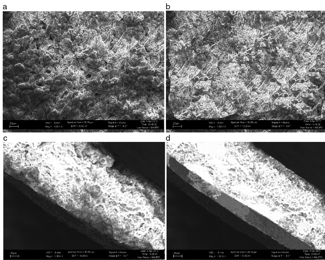
Fig. 5 – SEM images of deposited anode under different \text{N}_2 conditions. (a) and (c) are top view and cross section of samples treated at 1.7 \times 10^{18} \text{ molecules cm}^{-2} \text{ s}^{-1} \text{N}_2 flux, respectively, (b) and (d) are top view and cross section of samples treated at 4.3 \times 10^{18} \text{ molecules cm}^{-2} \text{ s}^{-1} \text{N}_2 flux.
