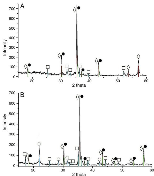
Fig. 4 – X-ray patterns of the 3\text{CoO} \cdot \text{Fe}_2\text{O}_3 \cdot \text{SiO}_2 sintered at 900 °C (A) and 1100 °C (B). ● – Cobalt ferrite \text{CoFe}_2\text{O}_4 – 79 – 1744; □ – Cobalt(II) Orthosilicate \text{Co}_2\text{SiO}_4 – 15 – 0865; ◇ – Magnetite \text{Fe}_3\text{O}_4 – 89 – 3854; ○ – Cristobalite \text{SiO}_2 – 89 – 3434.
