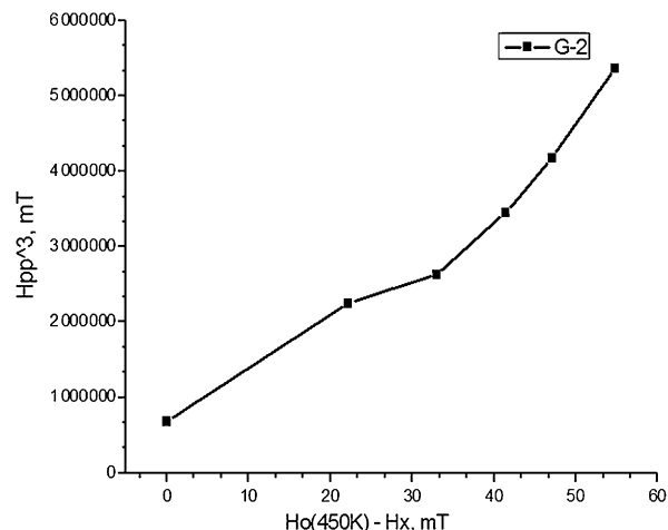
Fig. 6 – Dependence between the EPR signal band width for composition 2 sintered at 1100 °C, and its positional shift toward weaker magnetic fields.
