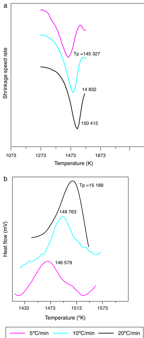
Fig. 8 – \theta to \alpha - \text{Al}_2\text{O}_3 maximum transformation peak of dilatometry derivative curves (a) and DTA curves (b) at various heating rates.
