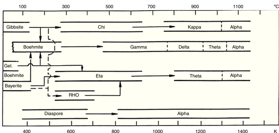
Fig. 1 – Transformation sequences of gibbsite ( \text{Al}(\text{OH})_3 ) to \alpha\text{-Al}_2\text{O}_3 [10].
