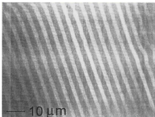
Figure 5 – Optical microscope image showing the microstructure of the \text{CaZrO}_3 – \text{CaSZ} eutectic. Light is guided by the \text{CaSZ} phase, appearing white in the image, as it presents a higher refractive index.
