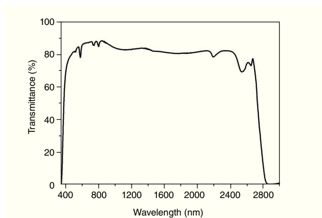
Figure 3 – Transmission spectra of a cook cover glass ceramics.
