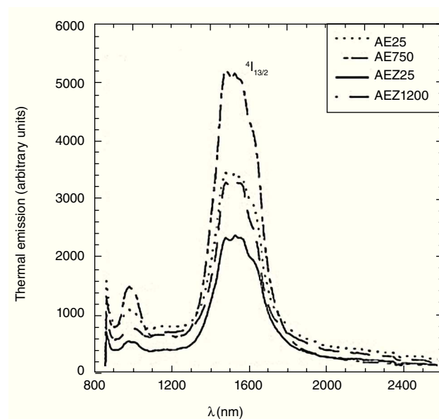
Figure 8 – Selective emission spectra of eutectics Al_2O_3-ErAl_2O_3 (AE) and Al_2O_3-ErAl_2O_3-ErSZ (AEZ) with coarse (AE25 and AEZ25) and fine (AE750 and AEZ1200) microstructures measured at 1600^\circ C from Mesa et al. 19
