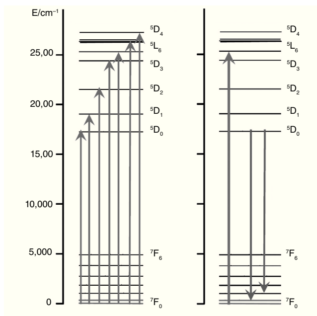
Figure 4 – Electronic states of the \text{Eu}^{3+} showing the light absorption bands (left) and the luminescence bands (right).
