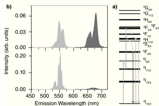
Figure 6 – a) Electronic levels of \text{Er}^{3+} showing a possible model for the two-photon IR absorption (blue lines) and the green and red emissions. b) Green and red emissions excited at the wavelengths indicated in the figures.
