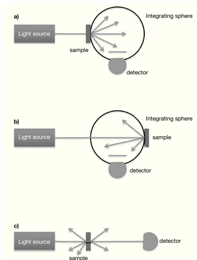
Figure 2 – Optical measurements. a) Total transmission, b) total reflectance, c) in-line transmission (RIT).
