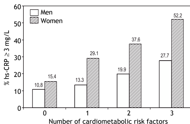
Figure 2. Prevalence of hs-CRP \geq 3 mg/L associated with the presence of fatty liver, adipose visceral fat \geq P_{75} ( AVF : men = 151.5 cm 3 , women = 122 cm 3 ) or HOMA-IR \geq P_{75} (men = 3.38, women = 3.66) and combination of two or three cardiometabolic risk factors. Trend in men p = 0.005 , in women p < 0.001 .
