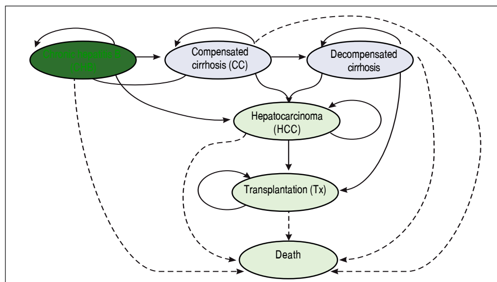
Figure 1. Markov diagram.
