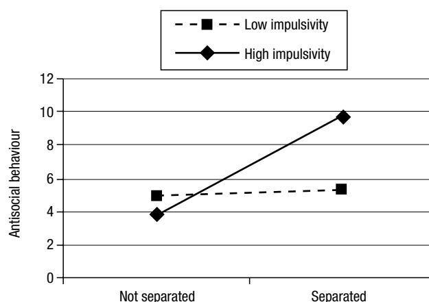
Figure 1 Impulsivity x separation interaction.
