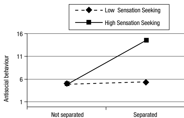
Figure 2 Sensation-Seeking x separation interaction.
