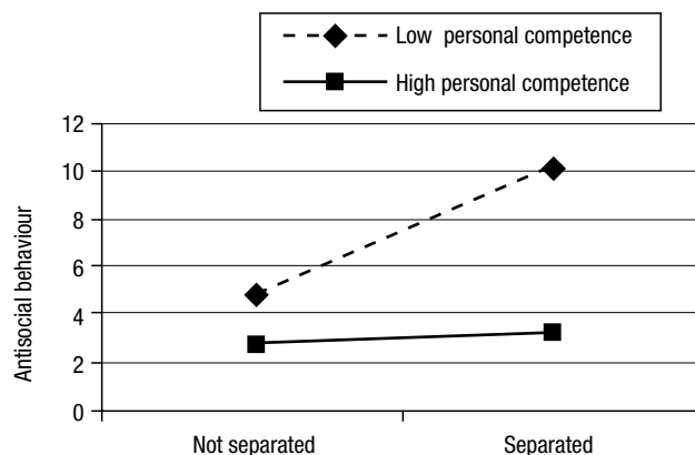
Figure 3 Personal competence and separation interaction.
